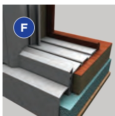
Insulated Sill
