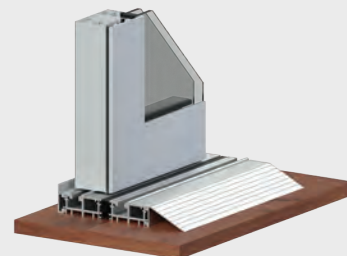
Multi-slide and Lift & Slide 1-1/8" standard sill
