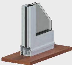
Bi-fold 1-1/8" standard sill
