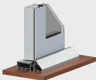
In-swing 1-1/4" standard sill
